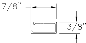
SASH STILE REINFORCEMENT 731-A ALUMINUM 6063-T5
