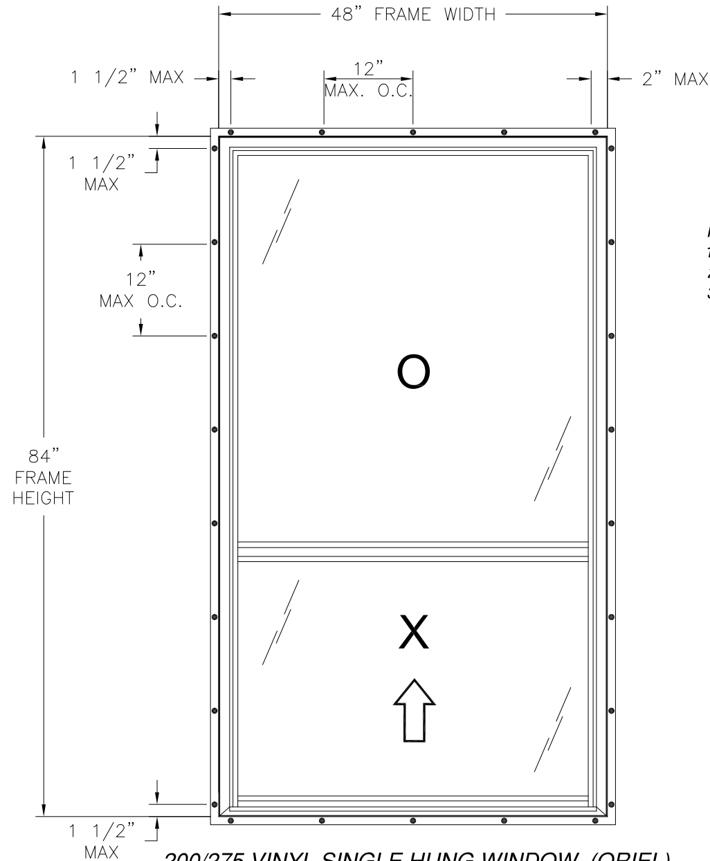
200/275 VINYL SINGLE HUNG WINDOW (ORIEL) EXTERIOR VIEW
